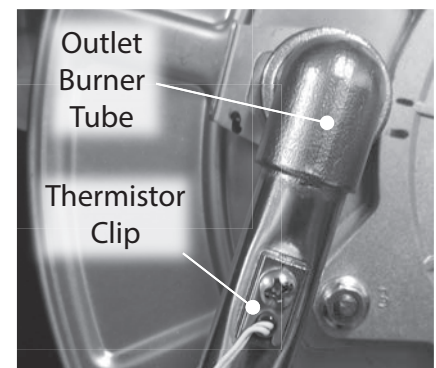
Figure 264 - Thermistor Clip, Outlet Burner Tube
