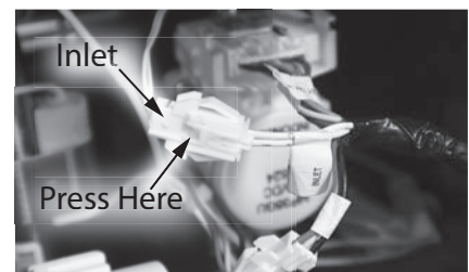
Figure 56 - Inlet harness disconnect instructions
