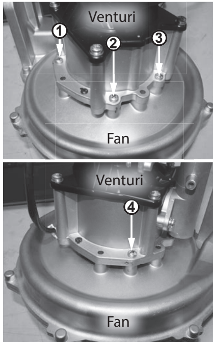
Figure 104 - Locate venturi and fan screws
