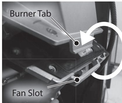
Figure 157 - Burner tab and fan slot
