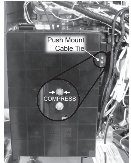
Figure 49 - Locating the push mount connector
