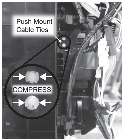
Figure 25 - Push mount cable tie removal.
