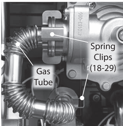
Figure 259 - Spring Clips (18-29), Gas Tube
