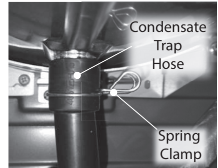
Figure 263 - Spring Clamp, Condensate Hose
