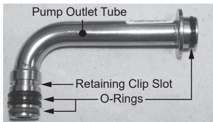
Figure 185 - Pump outlet tube O-rings
