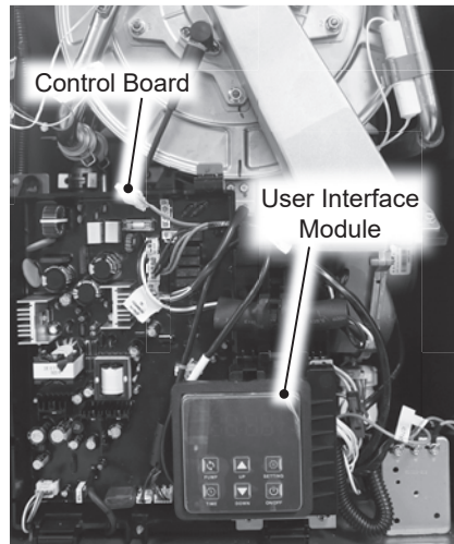
Figure 17 - User Interface Module
