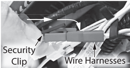
Figure 38 - Secure wiring with security clip
