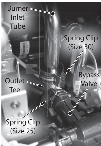
Figure 246 - Remove two spring clips from outlet tee
