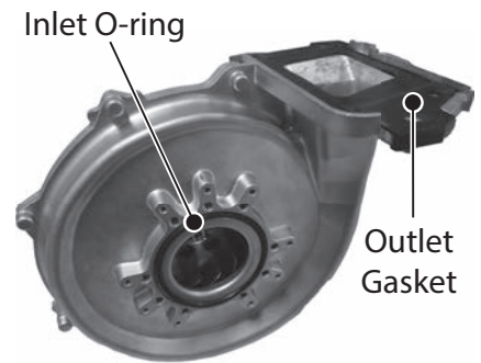
Figure 91 - Install inlet O-ring and outlet gasket to new fan assembly
