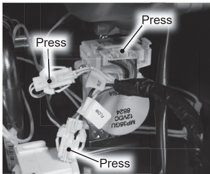
Figure 217 - Locating wiring harnesses
