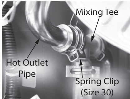
Figure 241 - Mixing tee location
