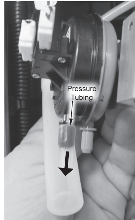
Figure 71 - Removing the pressure tube
