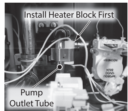
Figure 37 - Install pump outlet tube heater block
