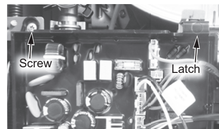
Figure 245 - Control board location
