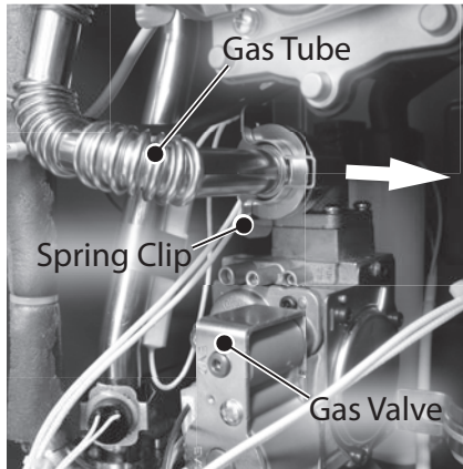
Figure 87 - Remove gas tube spring clip
