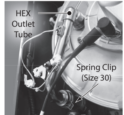
Figure 138 - Remove spring clip securing HEX outlet tube
