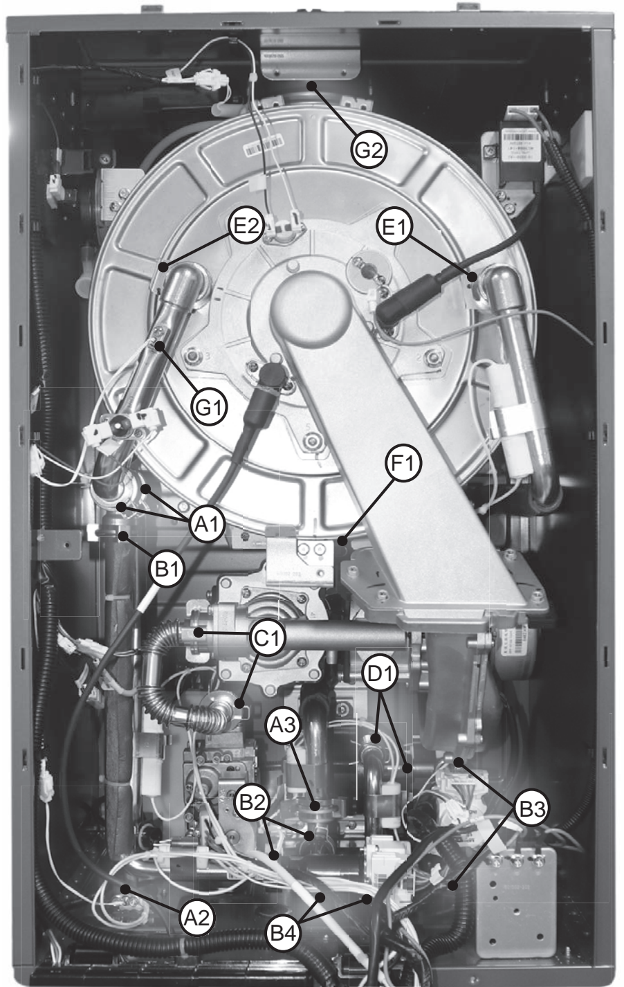
Figure 266 - Fastener Location Guide
