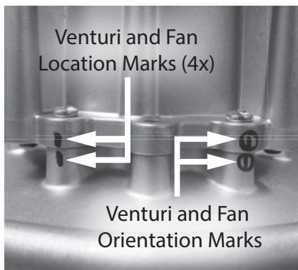
Figure 105 - Screw hole and orientation markings
