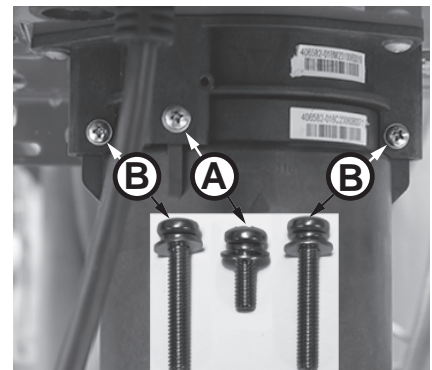
Figure 220 - Identify cartridge screws
