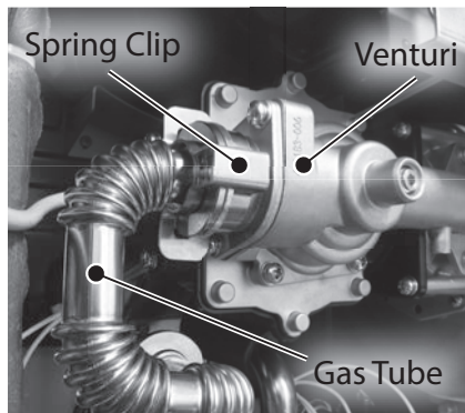
Figure 98 - Remove upper spring clip
