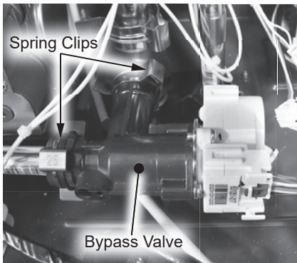
Figure 179 - Bypass valve location
