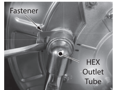
Figure 139 - Remove fastener securing HEX outlet tube
