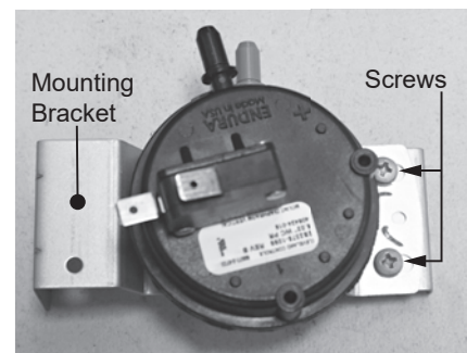
Figure 72 - Pressure switch mounting bracket
