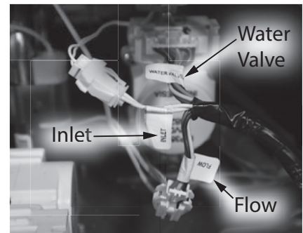
Figure 55 - Location of inlet flow module harnesses
