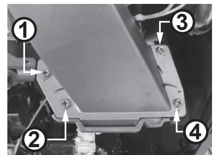
Figure 103 - Remove fan assembly screws
