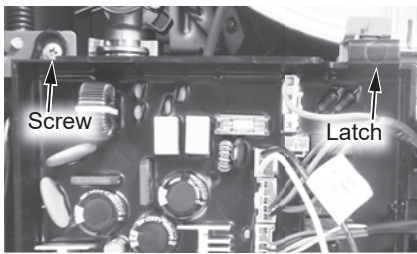
Figure 228 - Control Board screw location
