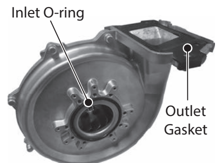
Figure 108 - Install inlet O-ring and outlet gasket to new fan assembly
