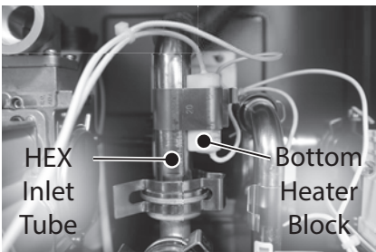
Figure 191 - Remove heater blocks from HEX inlet tube
