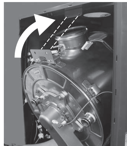
Figure 155 - Install heat exchanger to water heater
