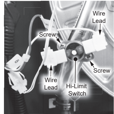
Figure 5 - Hi-Limit Switch (Manual)
