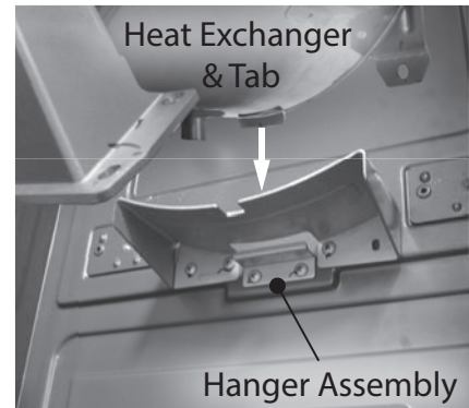
Figure 154 - Insert tab into hanger
