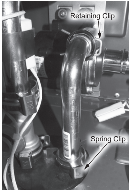
Figure 184 - Pump outlet tube location
