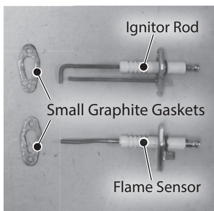
Figure 125 - Replace ignitor rod and flame sensor assemblies
