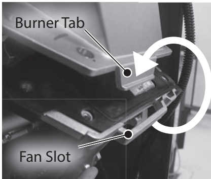
Figure 109 - Burner tab and fan slot
