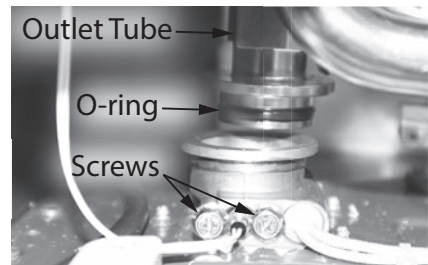
Figure 232 - O-ring location
