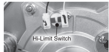
Figure 6 - Hi-Limit Switch (Burner Door)
