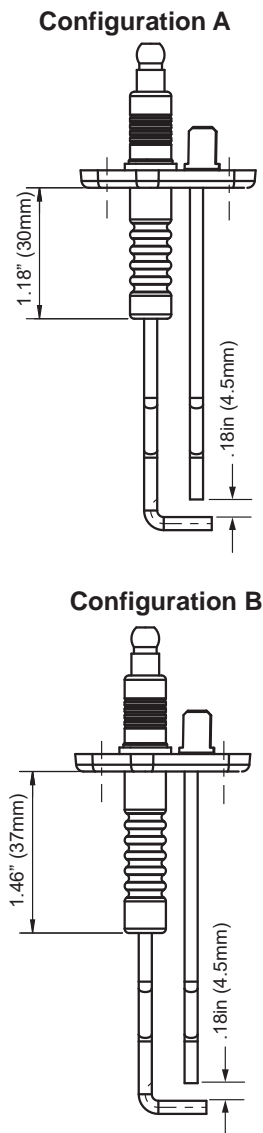
Figure 3: Ignitor rod configurations
