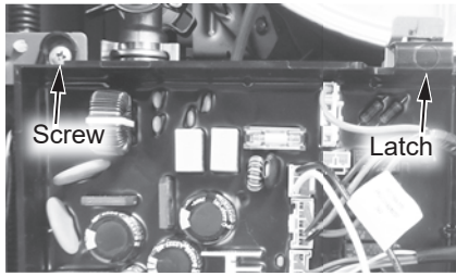
Figure 216 - Control board location
