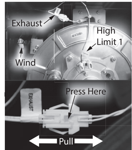
Figure 45 - First wiring harness bundle location
