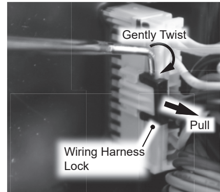
Figure 23 - Black harness lock removal
