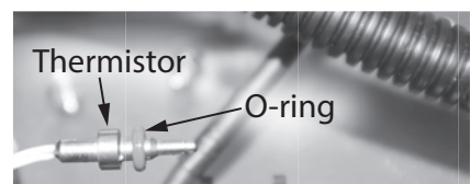
Figure 233 - Thermistor O-ring location
